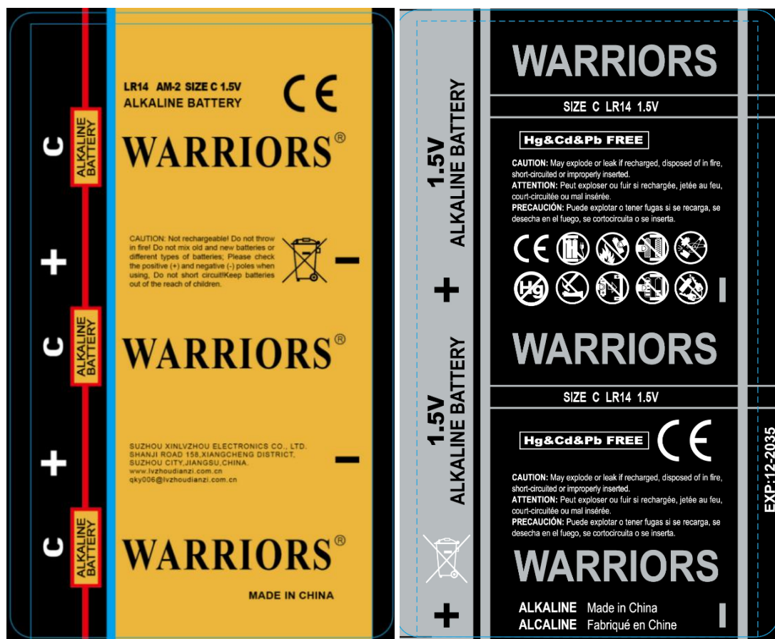
Battery jacket
