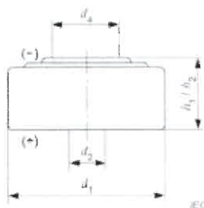
Figure 4 – Dimensional drawing: LR44
