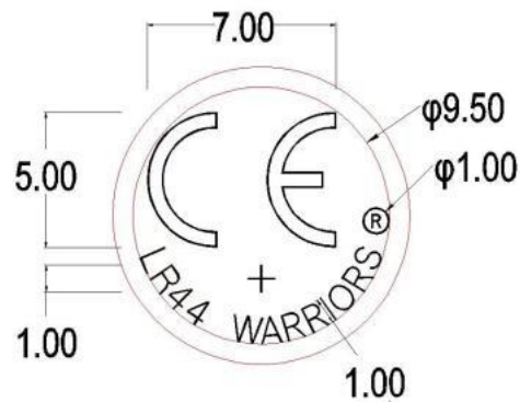
Battery jacket
