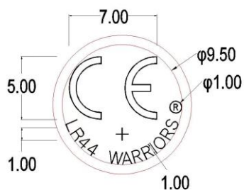
Battery jacket
